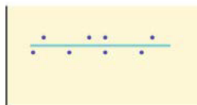
(c) Zero correlation
