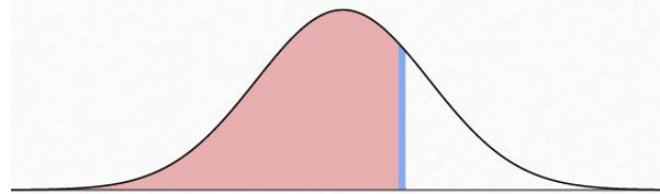
Standard Normal Distribution
