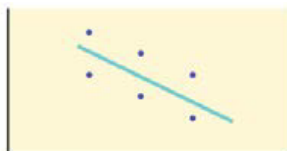
(b) Negative correlation
