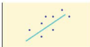
(a) Positive correlation
