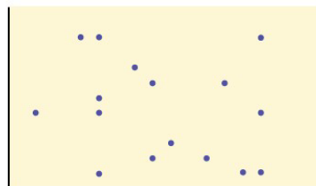
(b) No pattern
